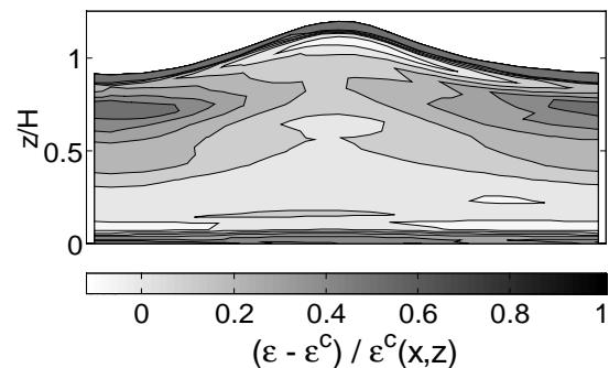
Figure 11: Wave-induced dissipation
