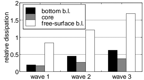
Figure 3: Integrated wave-induced dissipation by region normalized by current-only dissipation by region.
