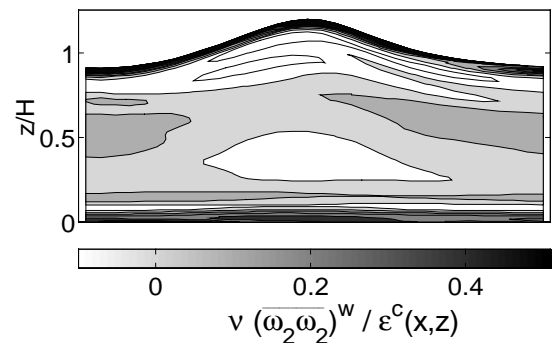
Figure 9: Wave-induced spanwise enstrophy
