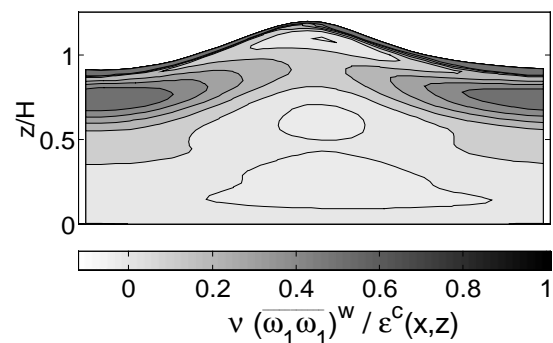
Figure 10: Wave-induced streamwise enstrophy
